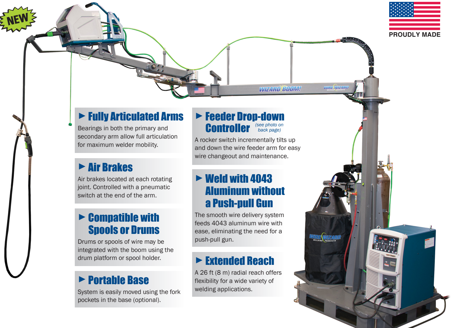
The ideal boom for aluminum welding applications
